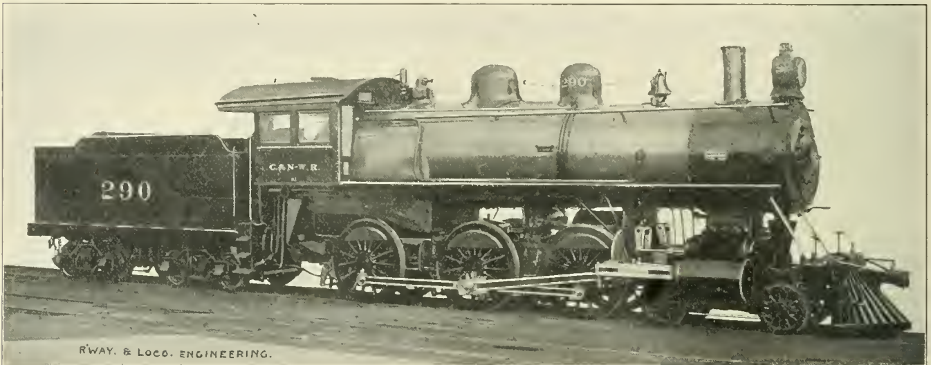
4-6-0 TYPE ENGINE FOR THE CHICAGO & NORTHWESTERN.
